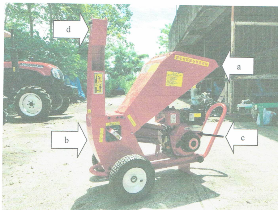
Figure 1. Parts of the WEIFANG 4" INLET Biomass Shredder powered by 5.7 kW Diesel Engine (a) Hopper, (b) Shredding Chamber, (c) Prime mover, and (d) Output chute
